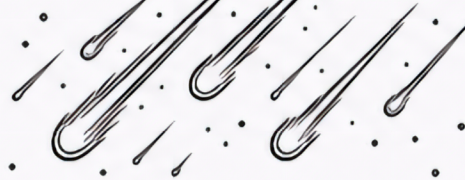
METEORS
