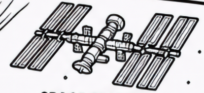
SPACE STATION
